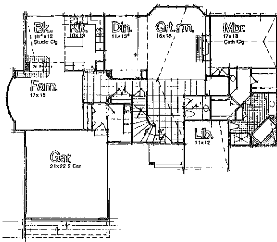
First Level Floor Plan
